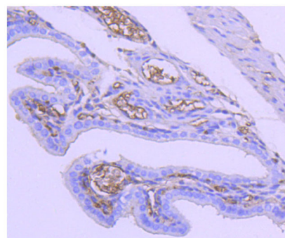
Fig. 2. Immunohistochemical analysis of paraffin-embedded mouse placenta tissue using anti-Tuberin antibody. counter stained with hematoxylin.
